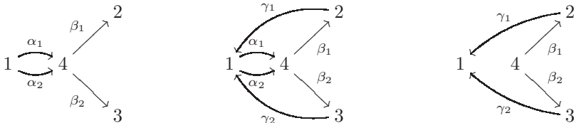
(a) The quiver of C , the relations are \alpha_1\beta_1 + \alpha_2\beta_1 = 0 , and \alpha_1\beta_2 - \alpha_2\beta_2 = 0 . (b) The quiver of B , and the potential W = (\alpha_1\beta_1 + \alpha_2\beta_1)\gamma_1 + (\alpha_1\beta_2 - \alpha_2\beta_2)\gamma_2 . (c) The quiver C' , the relations are \beta_1\gamma_1 and \beta_2\gamma_2 .
