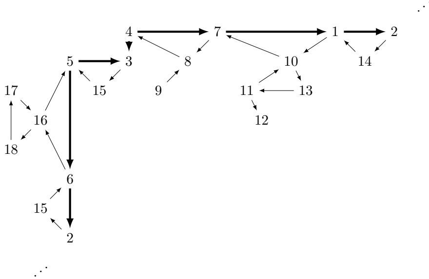
Figure 9: Mutation at 7: embedding
