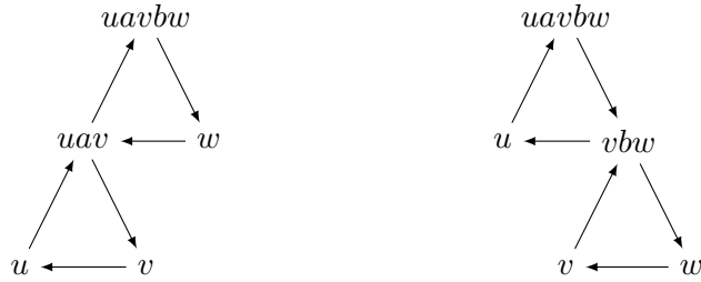
Figure 2: mutation of a continuant tree at a vertex different from the root
