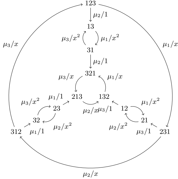
Figure 11: The function \delta
