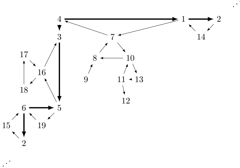
Figure 10: Mutation at 5: embedding
